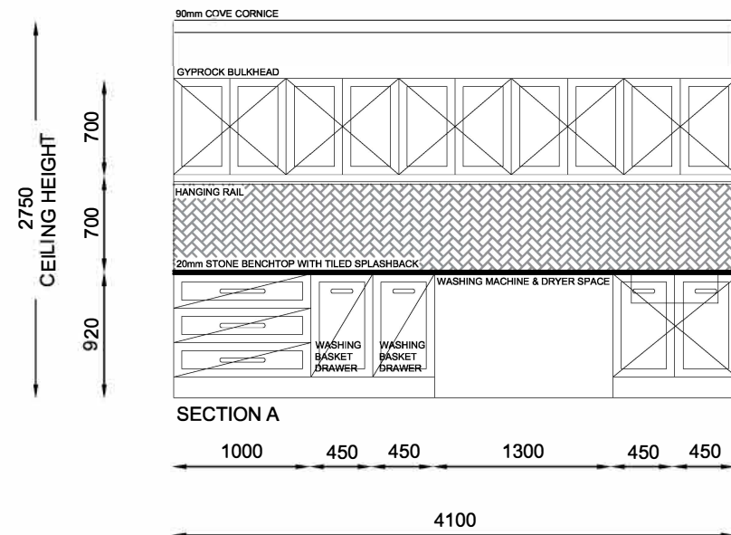
LAUNDRY ELEVATIONS
