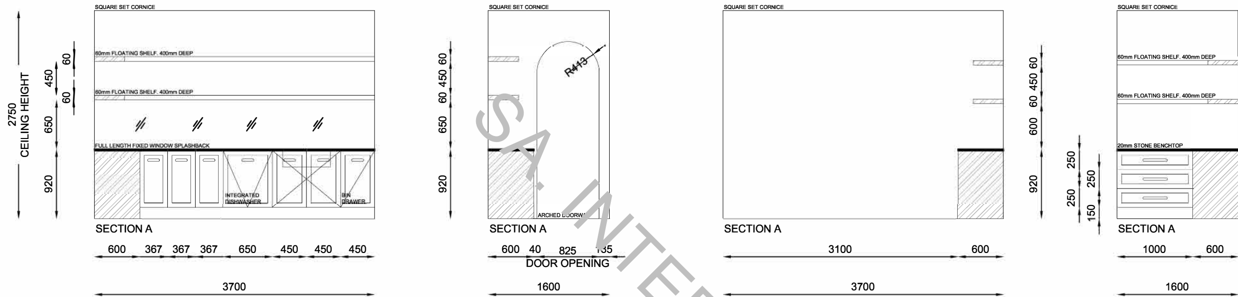
PANTRY ELEVATIONS
