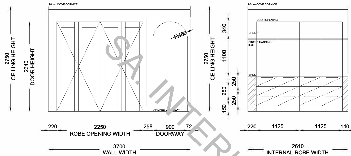
MASTER ROBE ELEVATIONS
